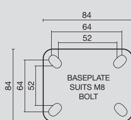
Baseplate for 50mm Low Profile Castors
