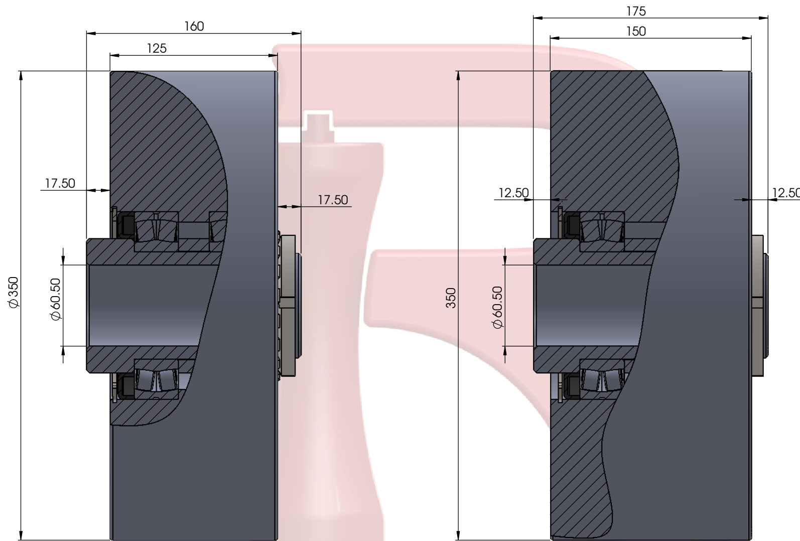
ST350X150 (80MM SPHERICAL ROLLER BEARINGS TO SUIT M60 PRECISION BOLT)
