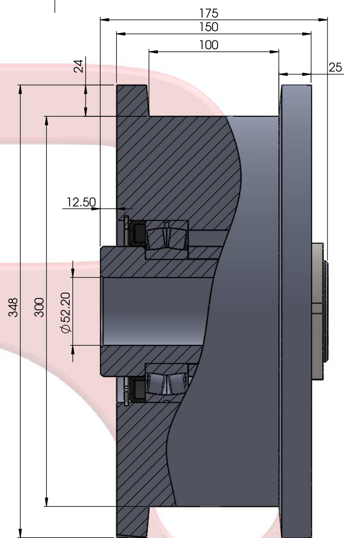
DFST300X100 (80MM SPHERICAL ROLLER BEARINGS TO SUIT M50 PRECISION BOLT)
