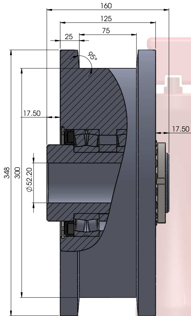
DFST300X75 (80MM SPHERICAL ROLLER BEARINGS TO SUIT M50 PRECISION BOLT)
