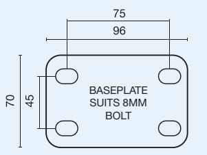
Baseplate for 75-125mm Swivel Castors
