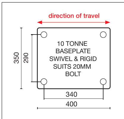
Twin Wheel baseplate dimensions
