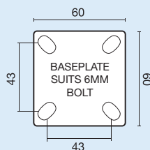
Baseplate for 50mm Swivel & Rigid Castors
