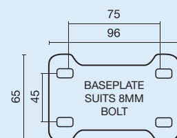
Baseplate for 75-100mm Rigid Castors
