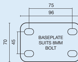
Baseplate for 75-100mm Swivel Castors
