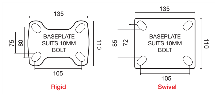
Baseplate dimensions & drilling patterns for 300 Series castors
