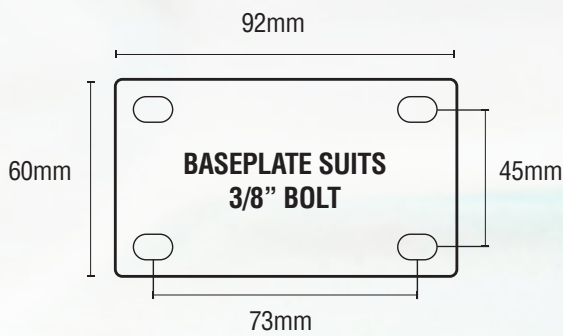
Baseplate dimensions & drilling patterns for adjustable height castor
